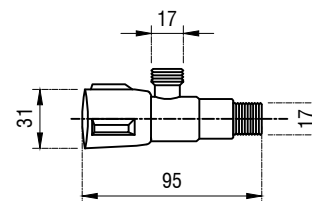
Angel Valve DCDT001-SV
