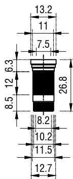
Flange for P-Trap D001SL-P
